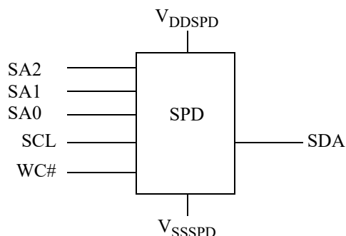
Figure 1 — Device Diagram
