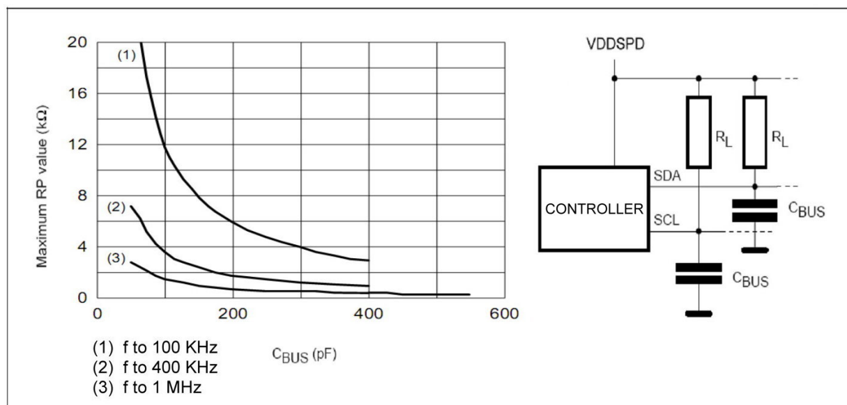
Figure 2 — Maximum R_L Value Versus Bus Capacitance ( C_{BUS} ) for an I 2 C Bus
