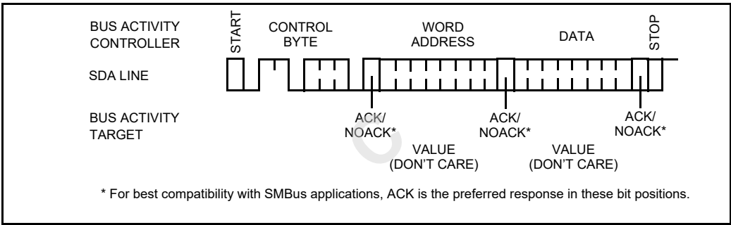
Figure 5 — Setting the Write Protection
