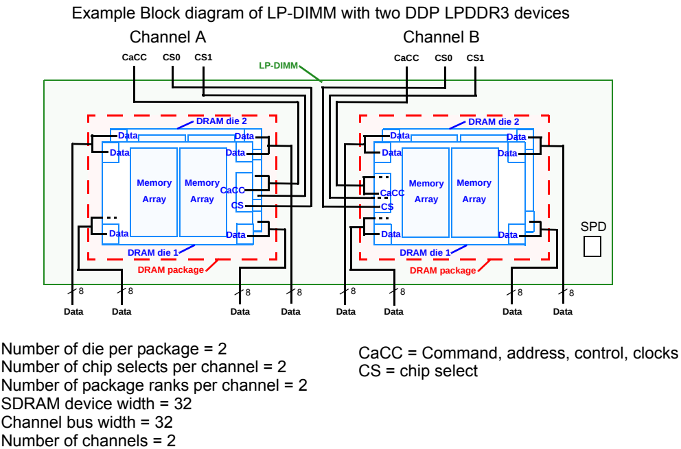
Figure 1 — Example Block Diagram of LP-DIMM with two DDP LPDDR3 Devices
